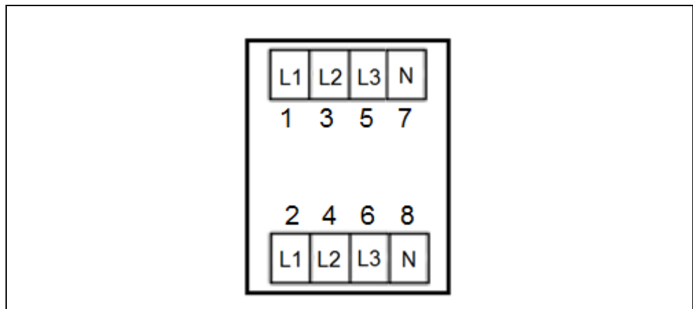
Abb. 6: Anschlüsse Schütz
